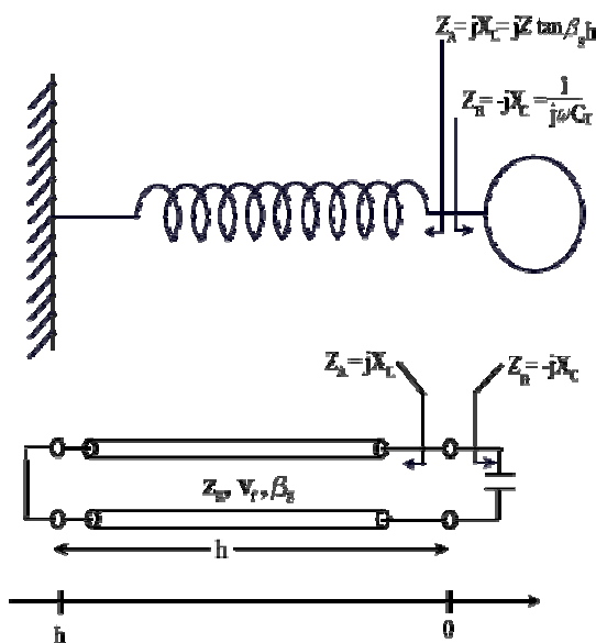
Figure 2. A capacitively tuned distributed resonator.
