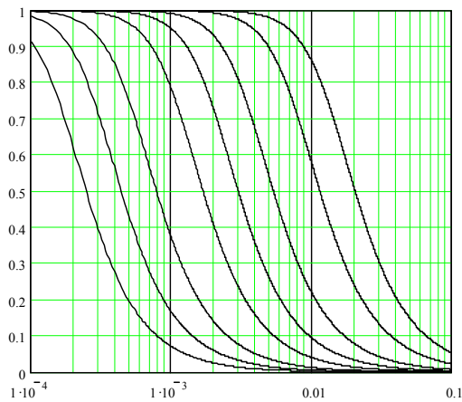
Fig. 1. V_f versus D/\lambda_o for coils of N = 1/s = 10,000; 5,000; 2,500; 1,000; 500; 250; 100; 50 turns/ \lambda_o , respectively (left to right).
