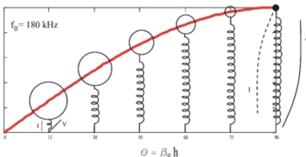
Figure 3. The solid curve is the voltage rise along a quarter wave resonator and shows the passage to lumped elements. As the load capacitance increases (with resonant frequency held constant), the transmission line must be shortened . . . until it behaves as a lumped inductance with a uniform current and linear voltage rise
