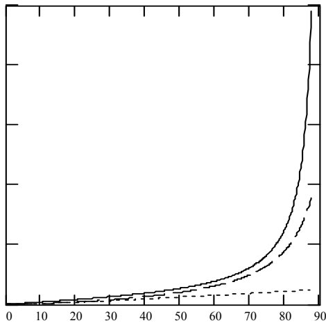
Figure 4. Graph of terminal point inductive reactance as a function of coil electrical length in degrees: true (solid), Medhurst's empirical parasitic element characterization (dashed), and conventional lumped element formula (dotted).
